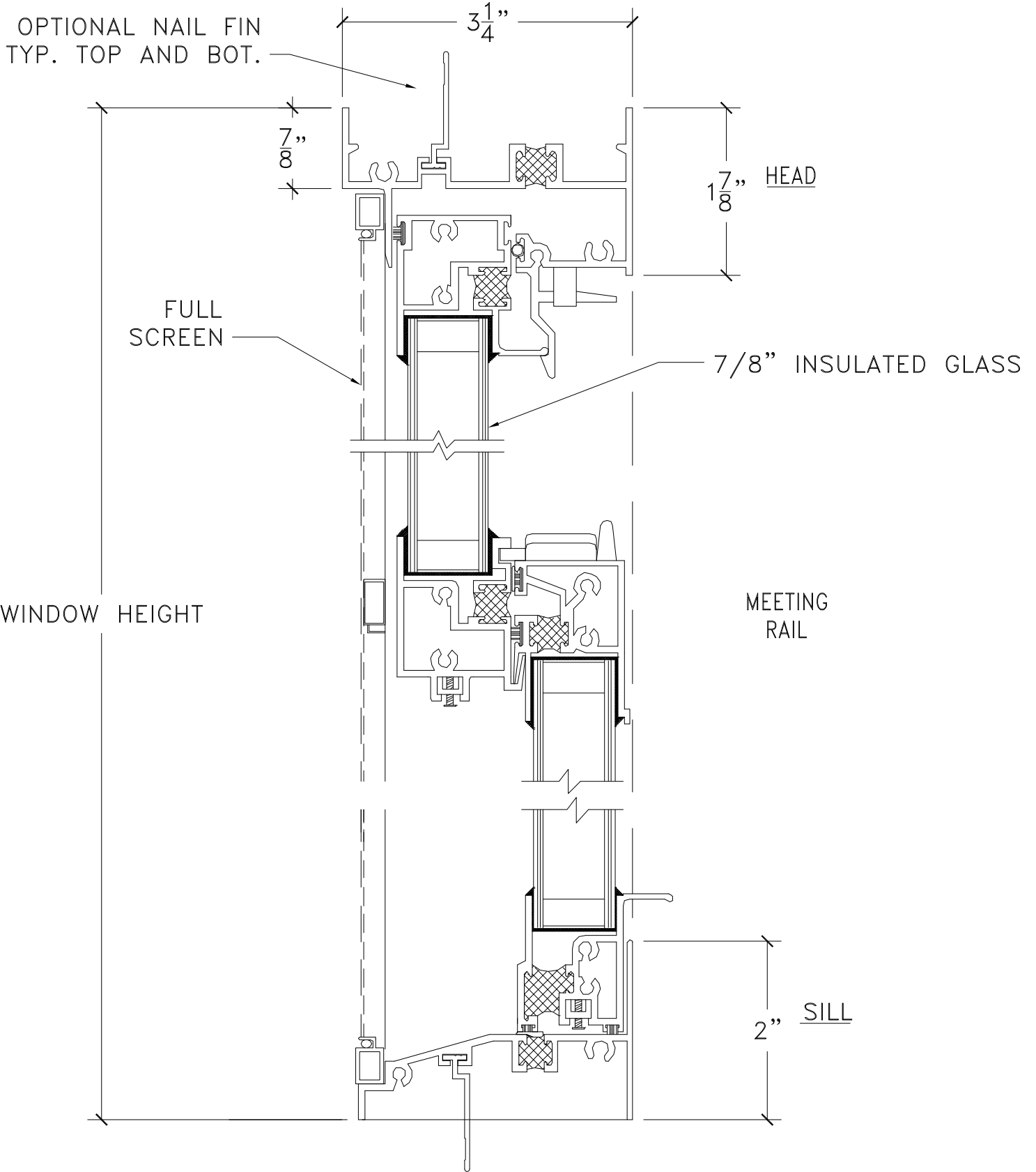
DOUBLE HUNG - TILT #8400 SERIES THERMAL BREAK ALUMINUM
